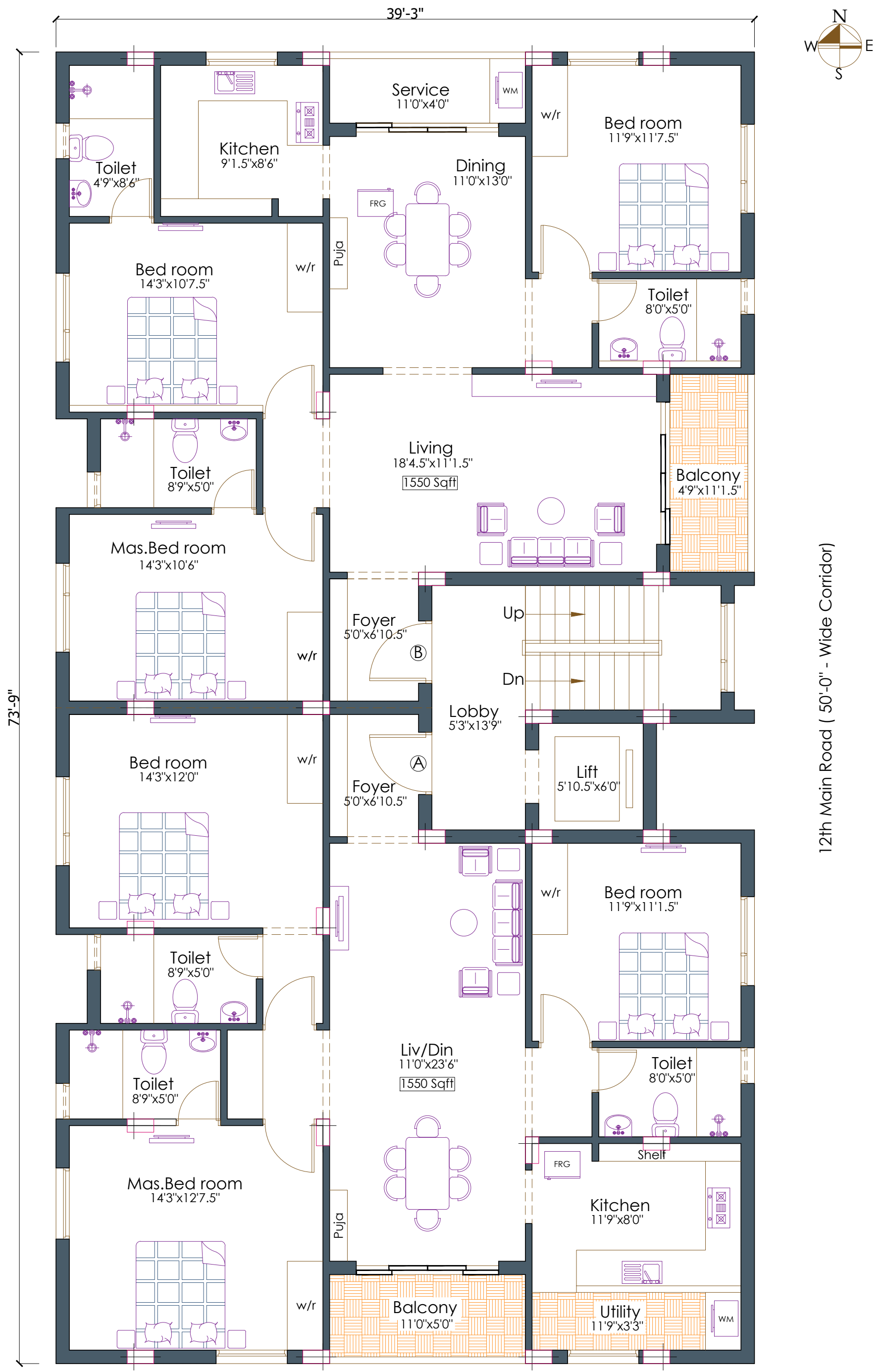
Typical Floor Plan (1st,2nd,3rd & 4th Floor)
