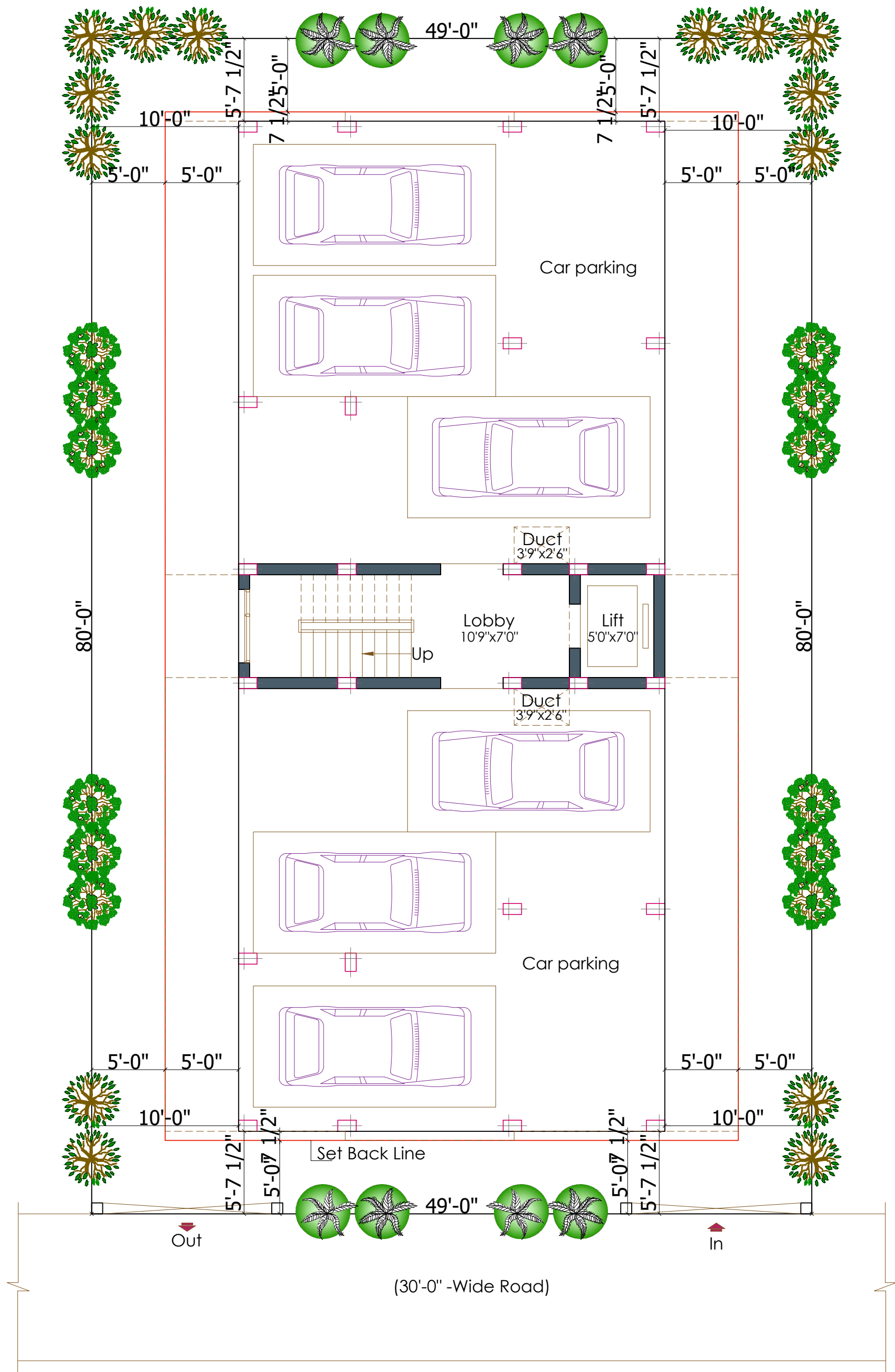
Site/Still Floor Plan
