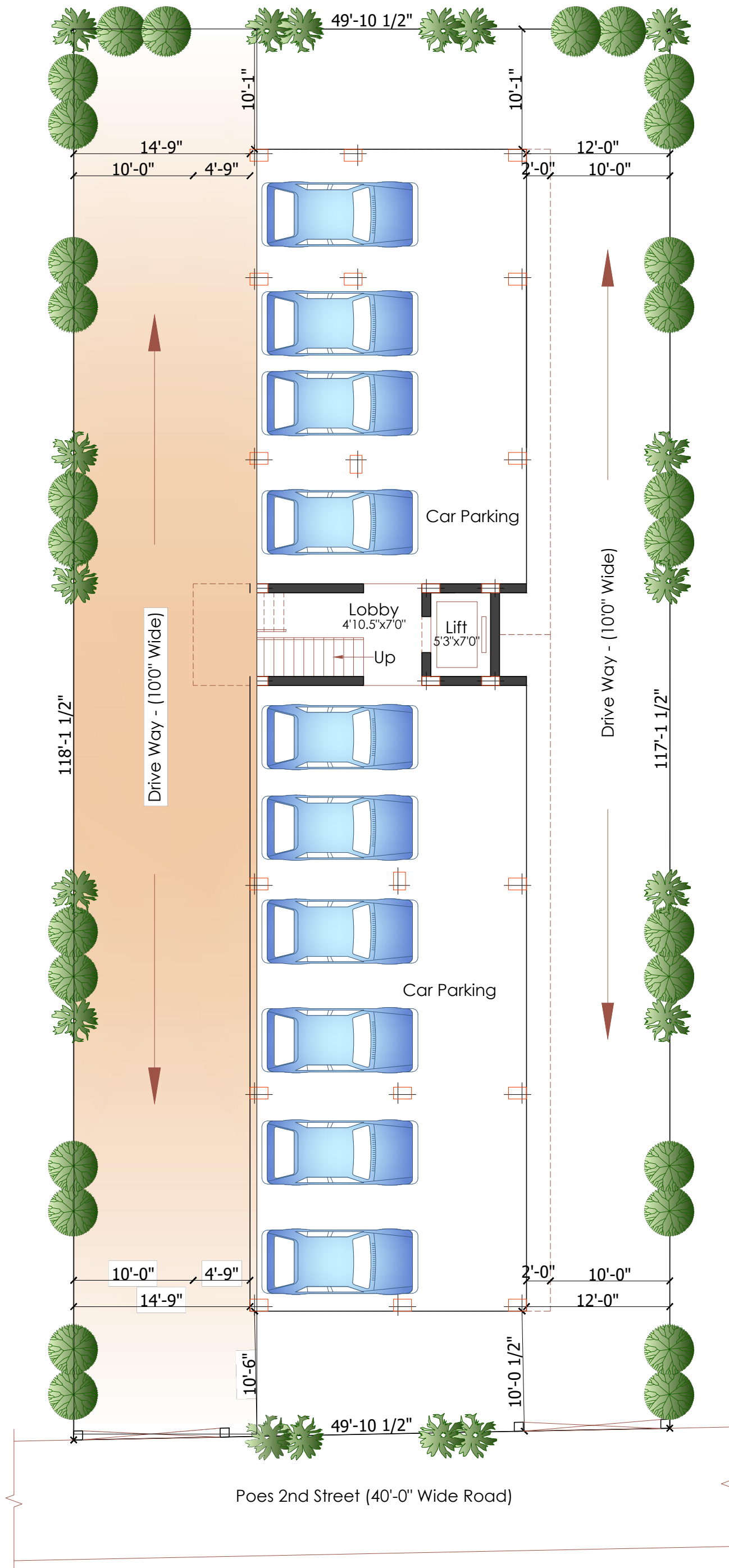
Site/Still Floor Plan
