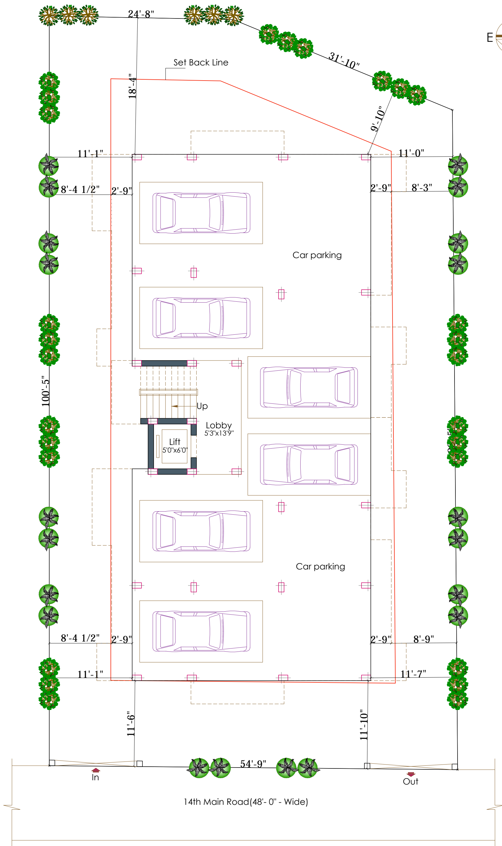
Site/Stilt Floor Plan
