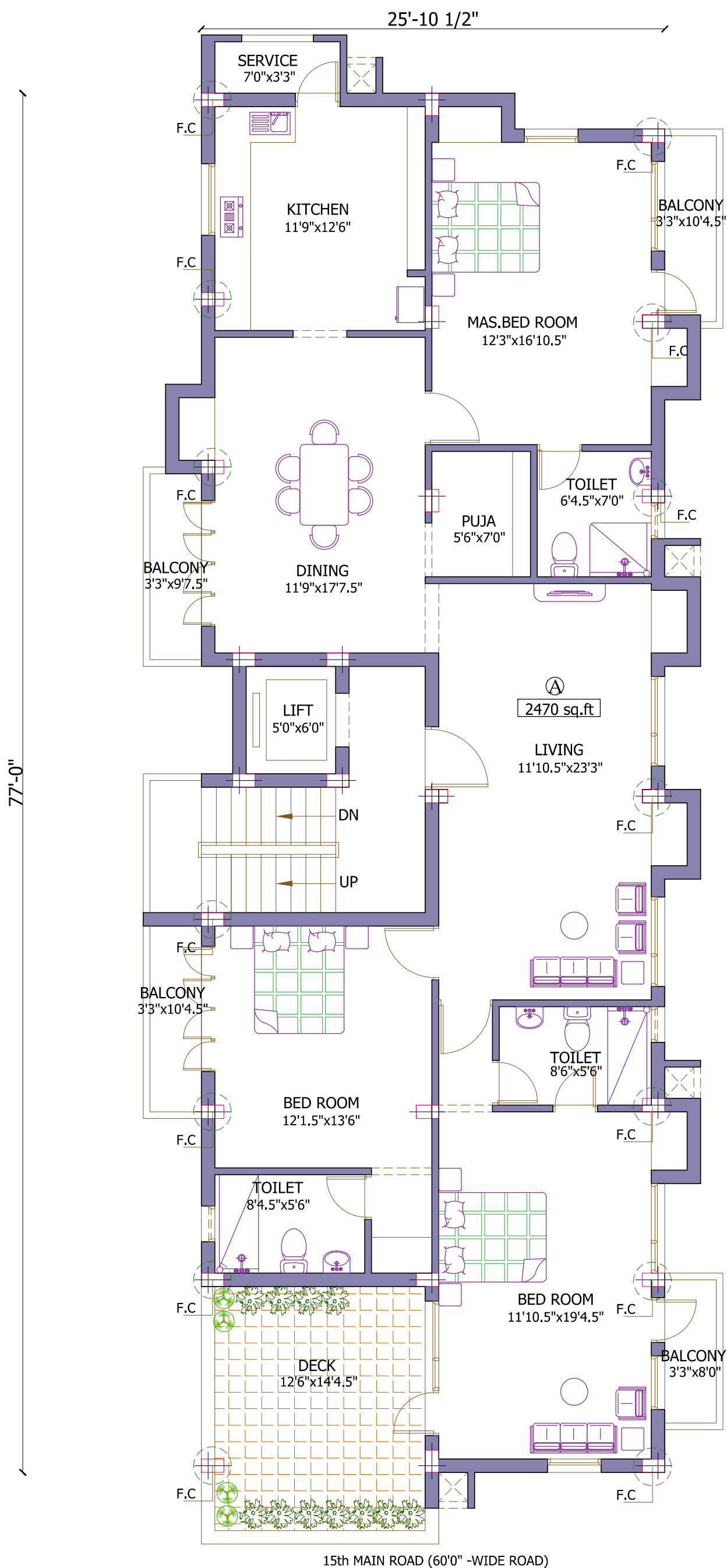
Typical Floor Plan (2nd & 3rd floor)
