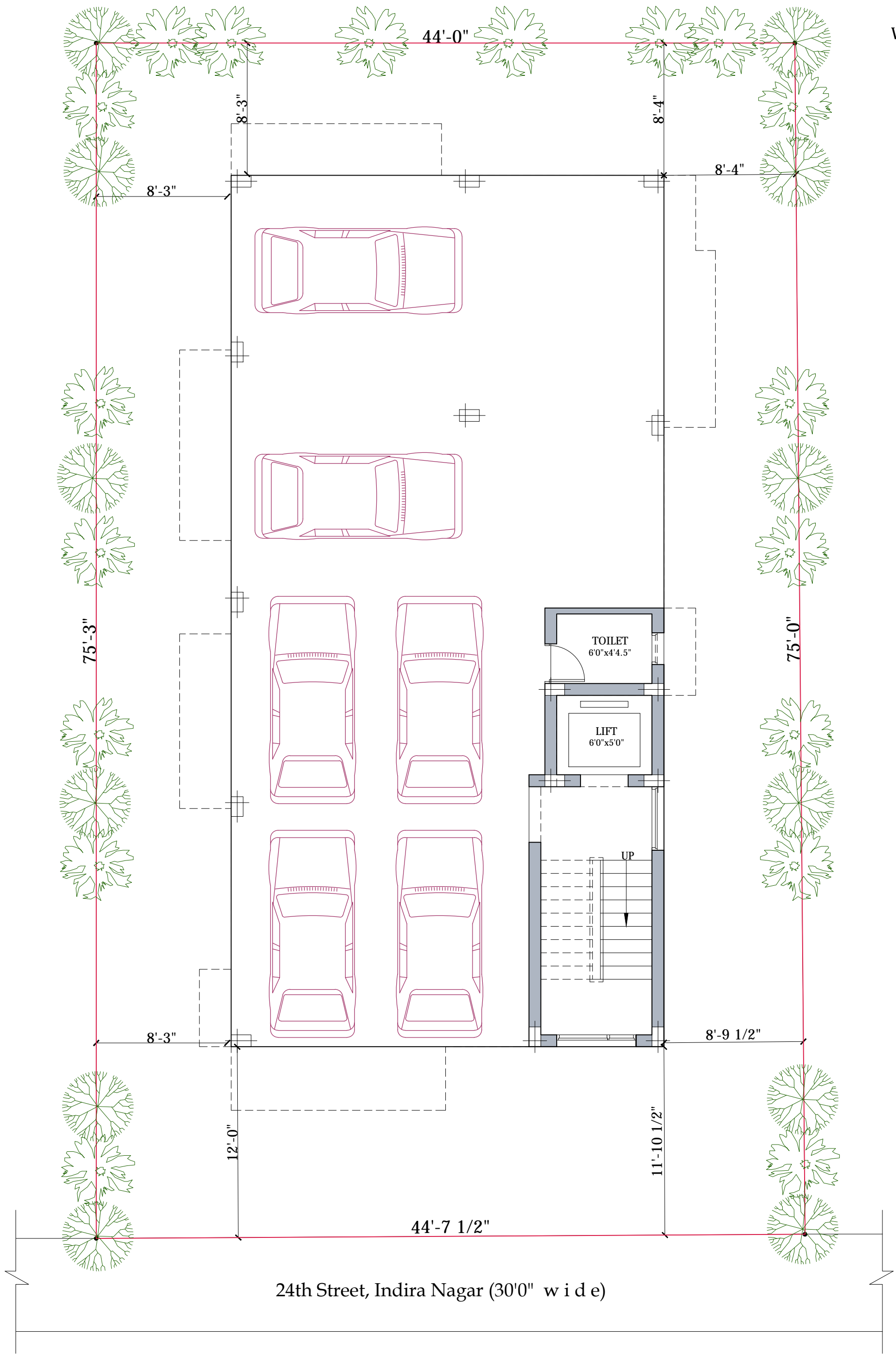
Site/Stilt Floor Plan
