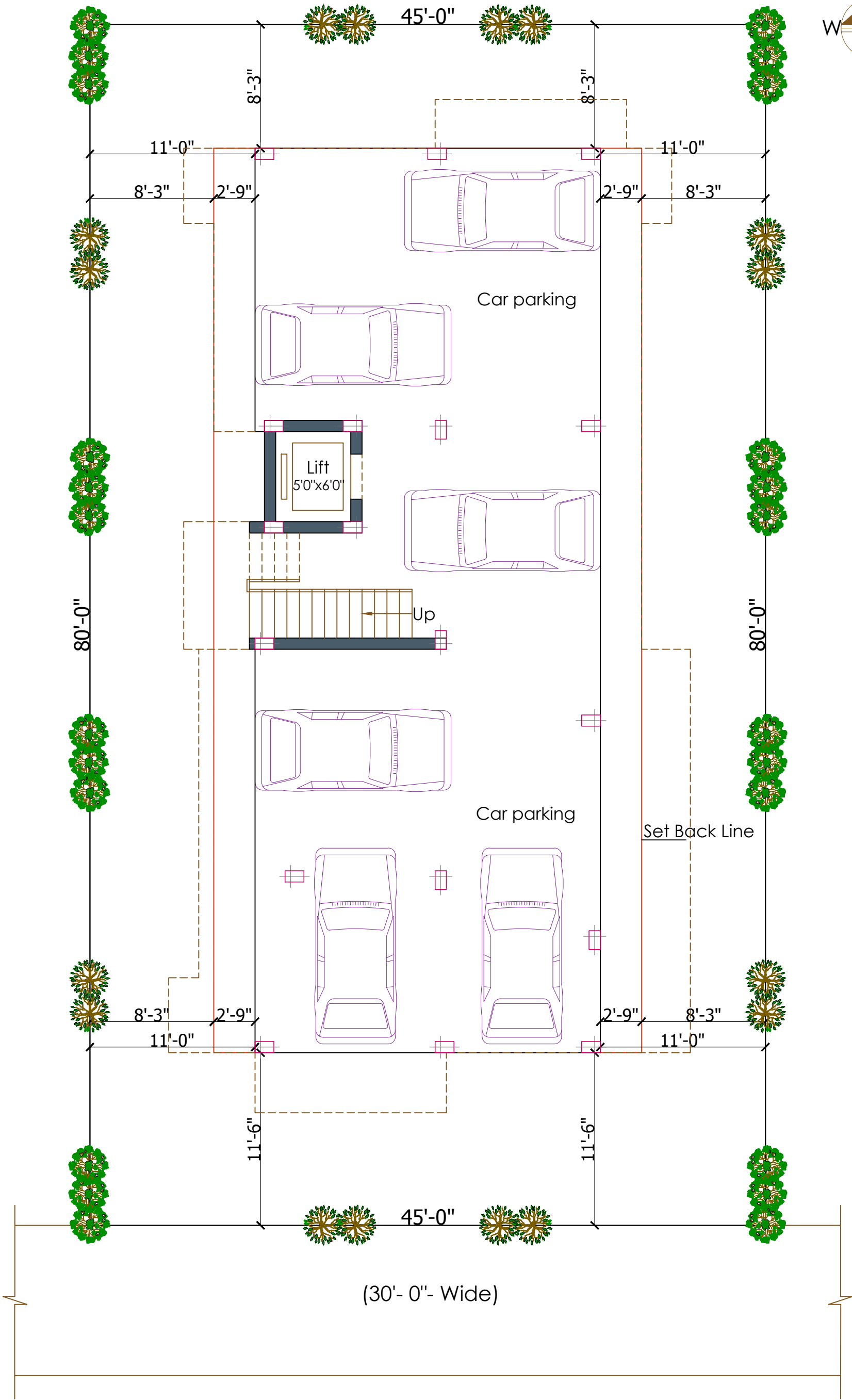
Site/Stilt Floor Plan
