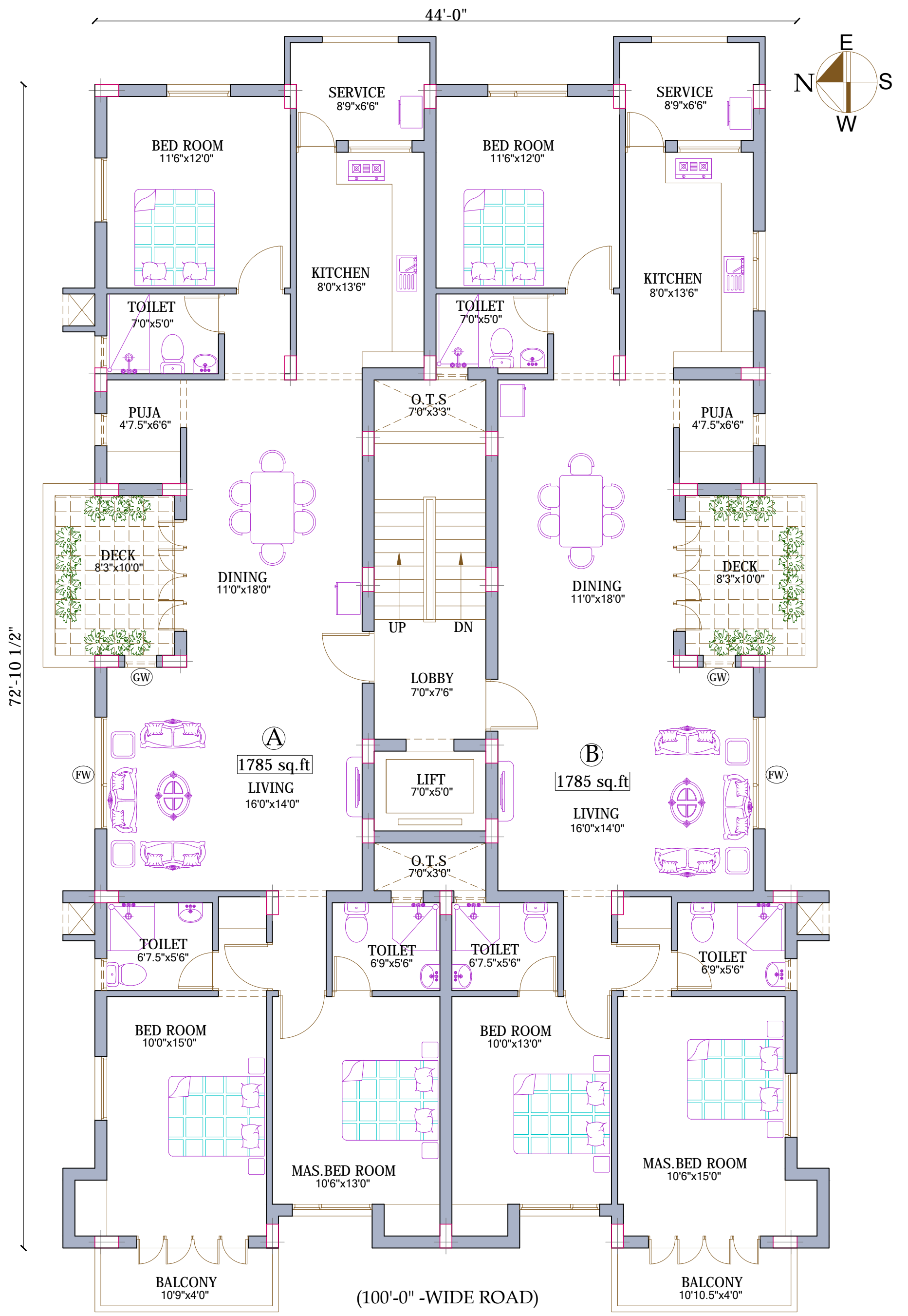
Typical Floor Plan (1st,2nd,3rd & 4th floor)
