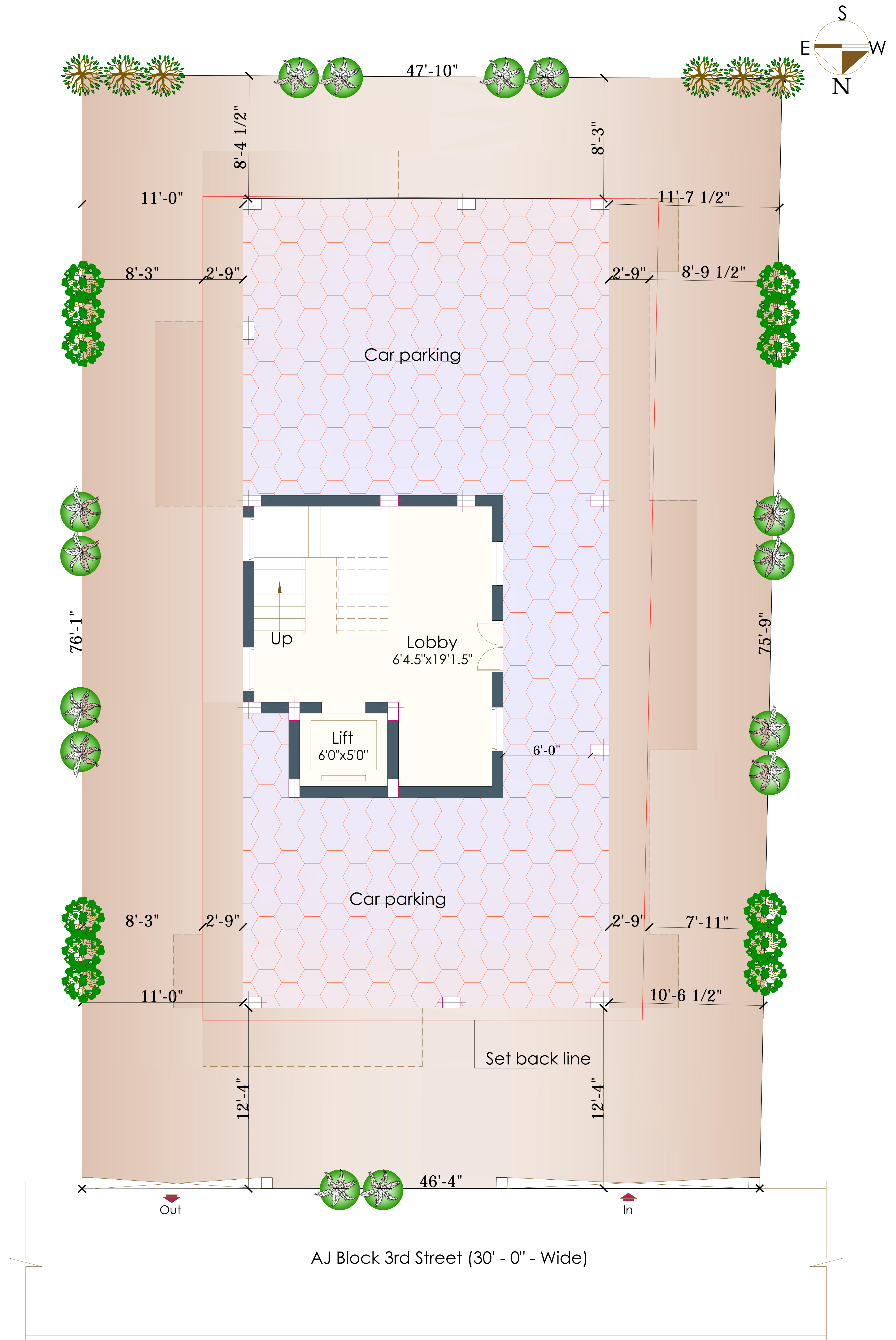
Site/Stilt Floor Plan
