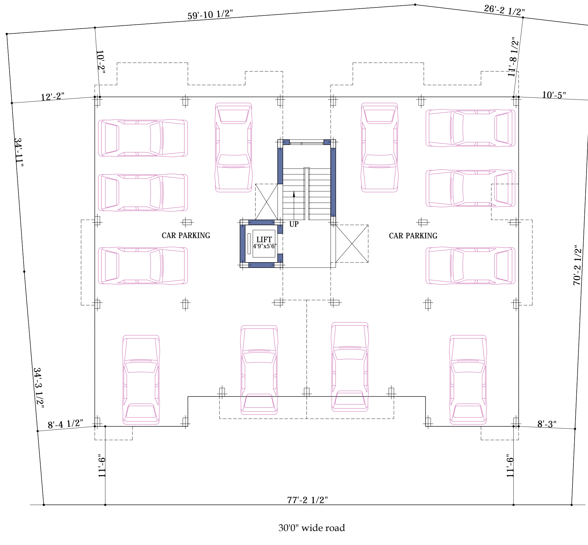
Site / Stilt Floor Plan
