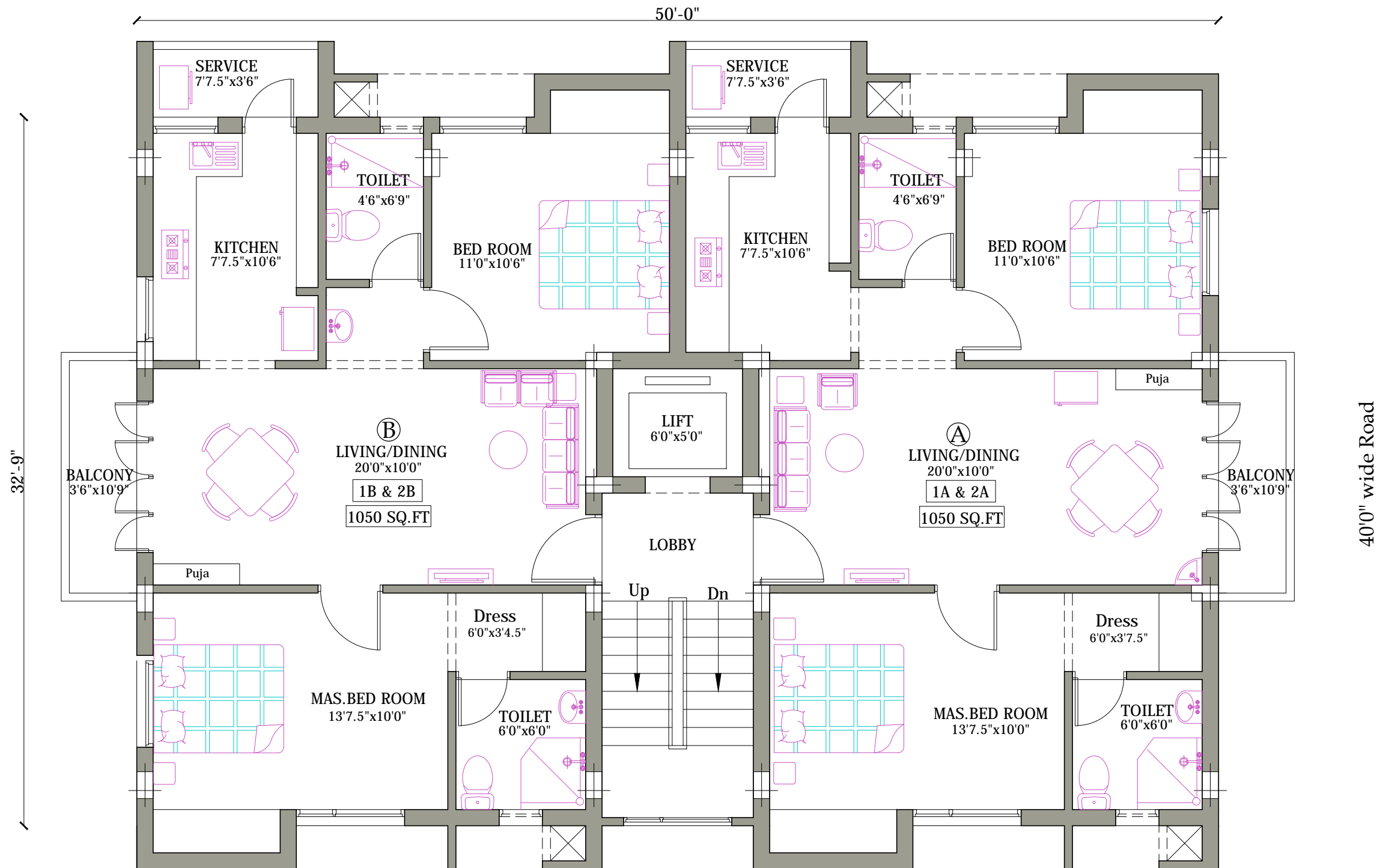
TYPICAL FLOOR PLAN (1st & 2nd Floor Plan)
