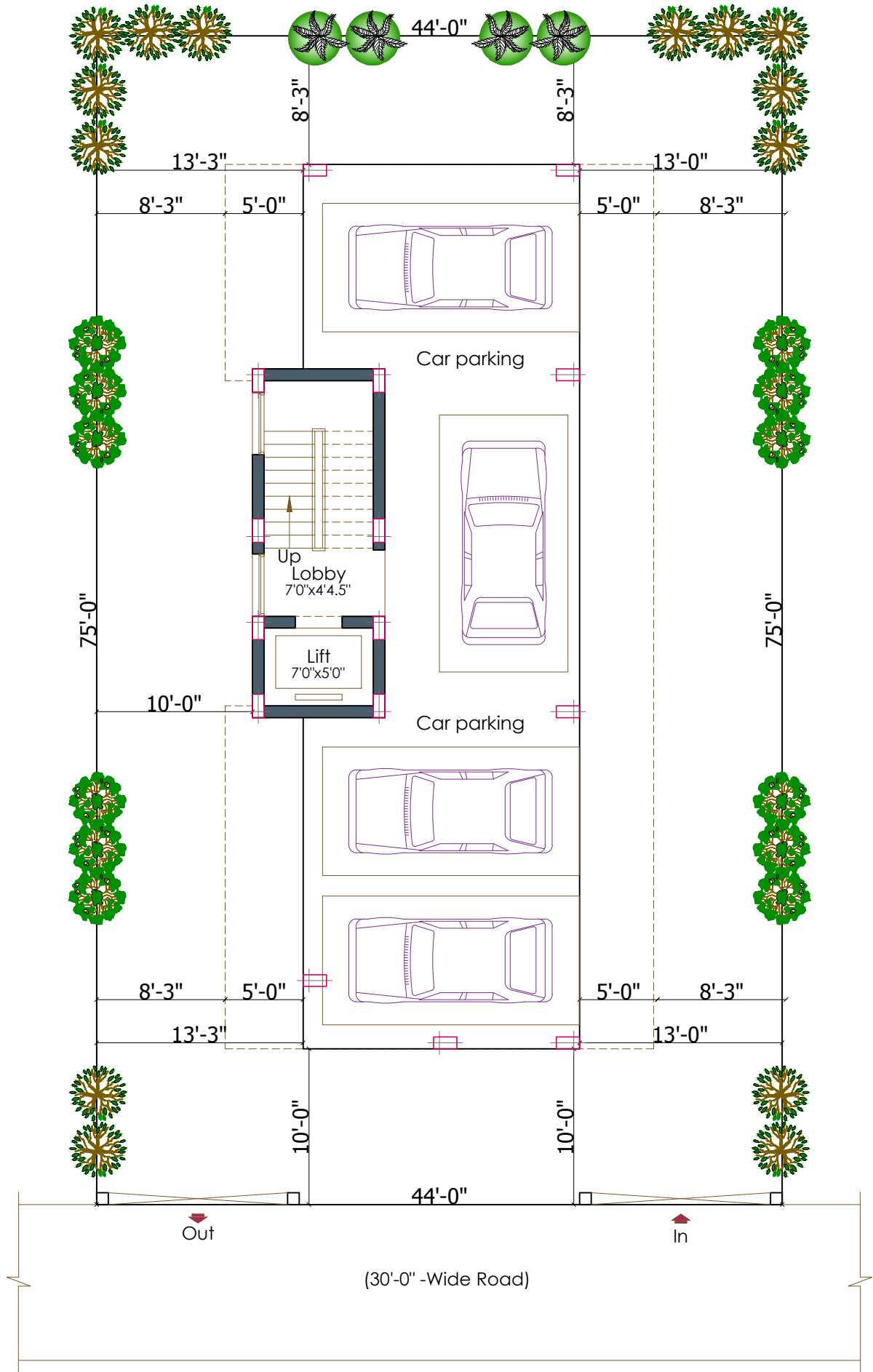
Site/Stilt Floor Plan
